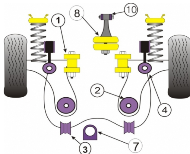
Golf 4 - 4motion
